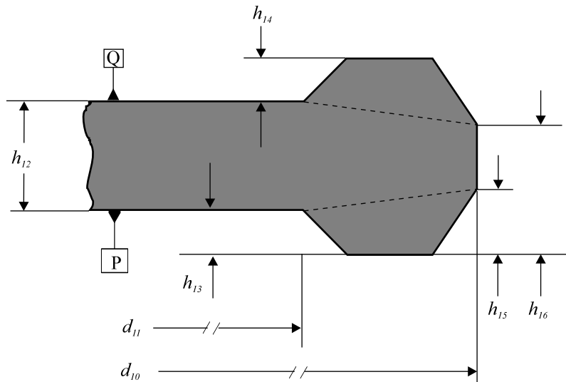
Figure 3 - Enlarged cross-section of the information area
